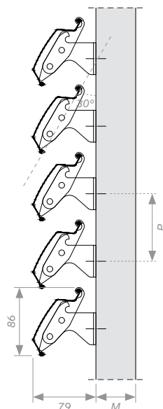
D 100 - 30°
